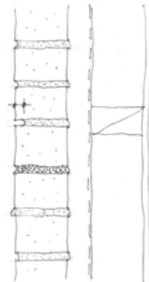
Figure 6 Recessed mortar joint too deep.
