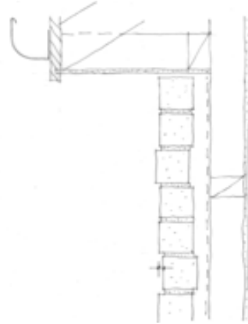
Figure 5 Bricks out of plumb in vertical plane.
